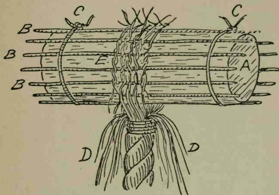
FIG. 90 A.—Making Flemish eye.
